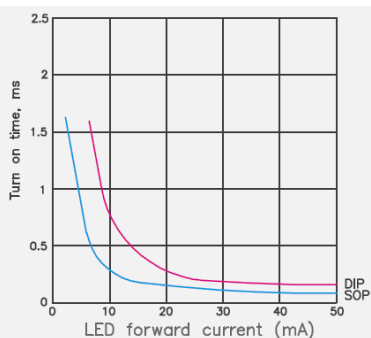
Turn on time vs. LED forward current
