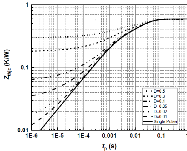
Fig. 8 • Maximum Transient Thermal Impedance, Z_{thjc} = f(t) , Parameter: D = t/T
