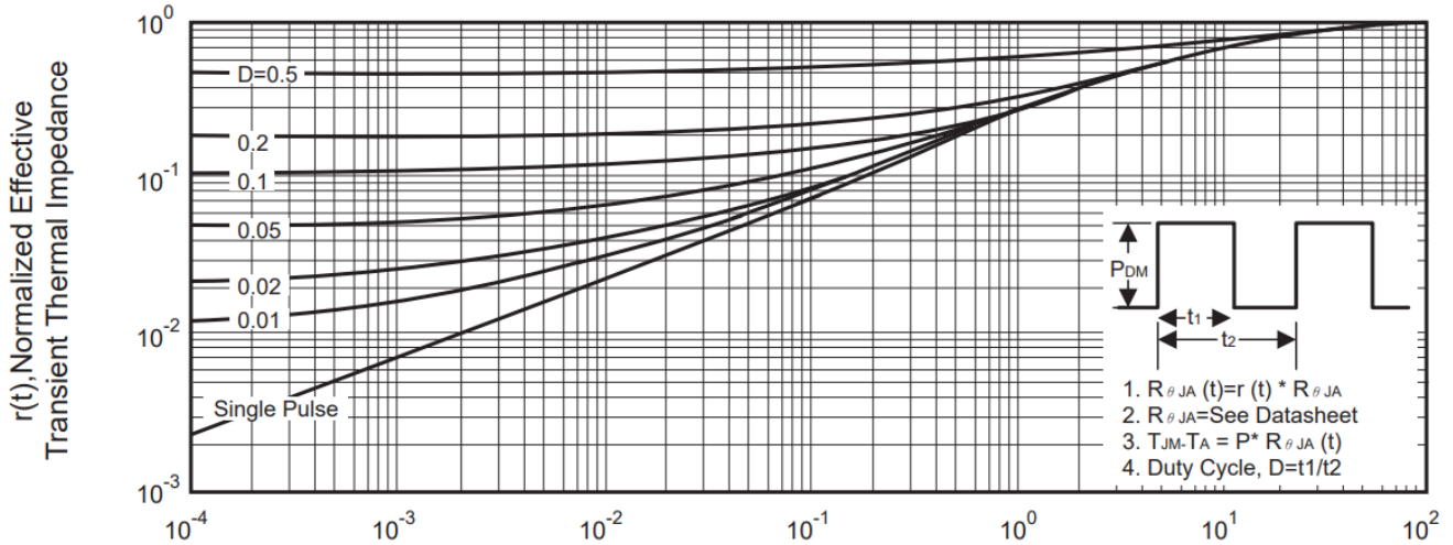
Fig. 12 ▪ Normalized Thermal Transient Impedance Curve
