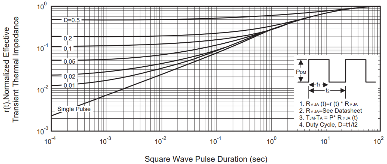
Fig. 12 ▪ Normalized Thermal Transient Impedance Curve
