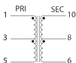
SCHEMATIC A
