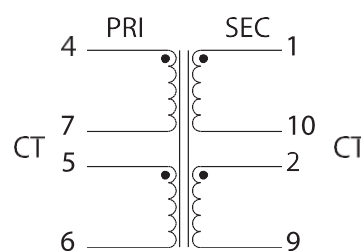
SCHEMATIC B
