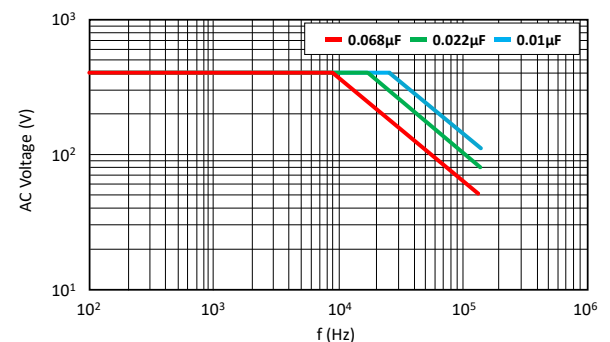
Fig. 8 • Max. RMS Voltage vs. Frequency • 1000V DC /400V AC
