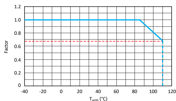
Fig. 12 • Max. AC Voltage vs. Temperature
