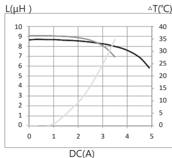
8. MTI-SDR0843A-8R2-T125
