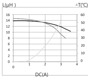
10. MTI-SDR0843A-150-T125
