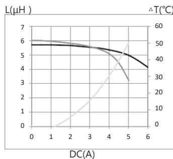
6. MTI-SDR0843A-5R6-T125
