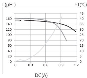
16. MTI-SDR0843A-151-T125
