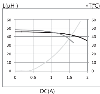
16. MTI-SDR0843A-151-T125
