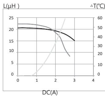
14. MTI-SDR0843A-680-T125
