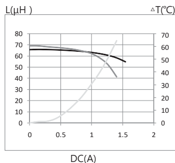
17. MTI-SDR0843A-221-T125
