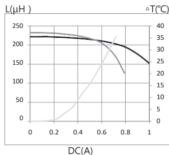
17. MTI-SDR0843A-221-T125
