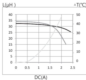
15. MTI-SDR0843A-101-T125
