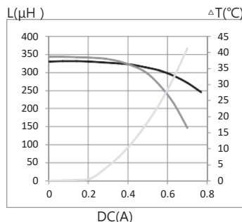
18. MTI-SDR0843A-331-T125
