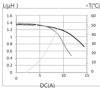
1. MTI-SDR0843A-1R2-T125
