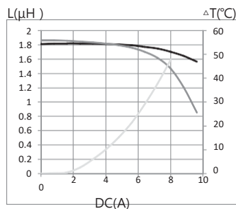
2. MTI-SDR0843A-1R8-T125
