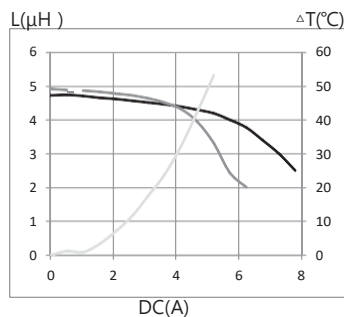
5. MTI-SDR0843A-4R7-T125
