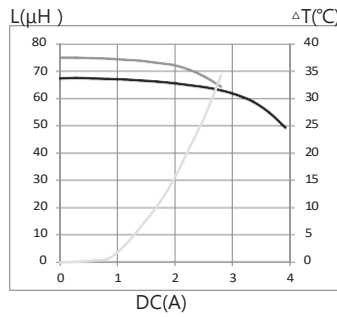
14. MTI-SDR1207A-221-T125
