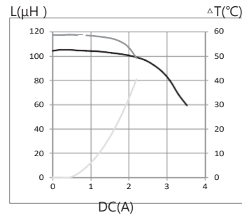
15. MTI-SDR1207A-331-T125
