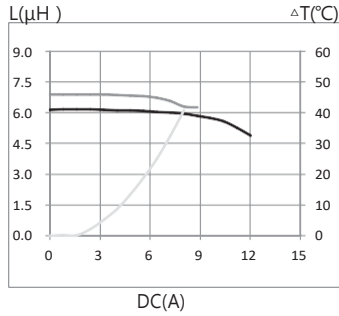
7. MTI-SDR1207A-150-T125
