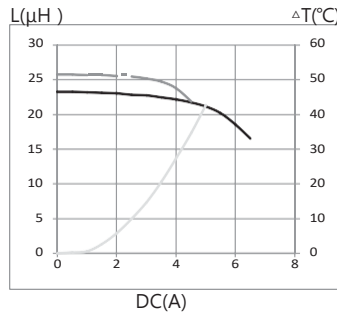
11. MTI-SDR1207A-680-T125
