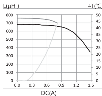
17. MTI-SDR1207A-681-T125
