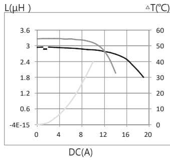
4. MTI-SDR1207A-6R2-T125
