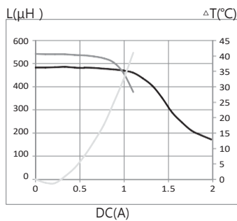
16. MTI-SDR1207A-471-T125
