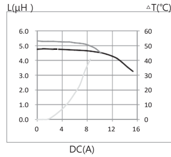
6. MTI-SDR1207A-100-T125
