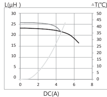
12. MTI-SDR1207A-101-T125
