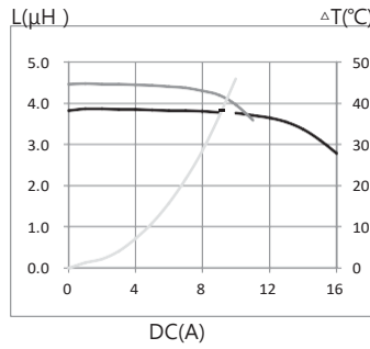
5. MTI-SDR1207A-7R5-T125
