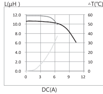
9. MTI-SDR1207A-330-T125
